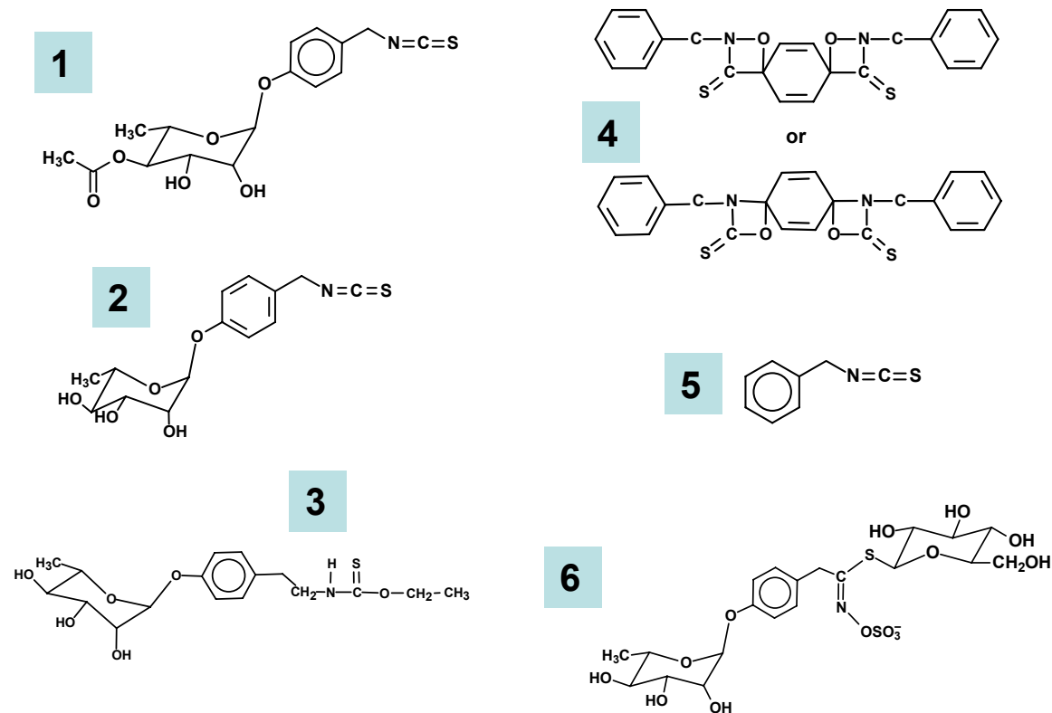
Figure 1. Structures of selected phytochemicals from Moringa spp.: 4-(4'- O -acetyl- \alpha -L-rhamnopyranosyloxy)benzyl isothiocyanate [1], 4-( \alpha -L-rhamnopyranosyloxy)benzyl isothiocyanate [2], niazimicin [3], pterygospermin [4], benzyl isothiocyanate [5], and 4-( \alpha -L-rhamnopyranosyloxy)benzyl glucosinolate [6]
