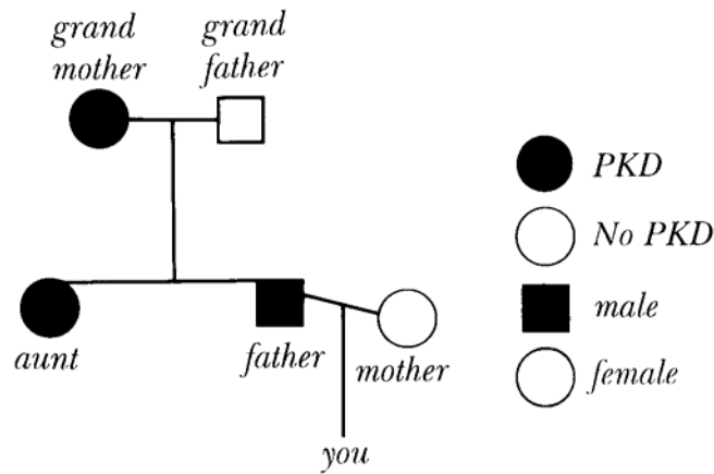
Example of an informative family for gene linkage analysis
